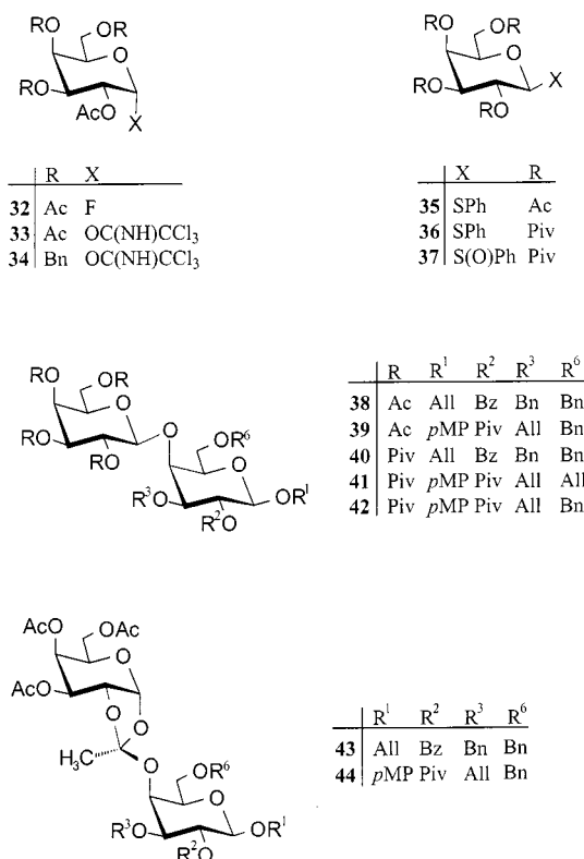
Scheme 3. Evaluation of galactosyl donors 32–37 for generation of \beta(1\rightarrow4) -galactobiosides by coupling with acceptors 23 , 27 , and 31 . Only the pivaloylated donors 36 and 37 proved free of orthoester formation, yielding disaccharides 40–42 efficiently (cf. Table 1)
