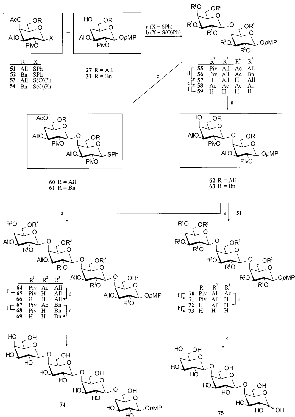
Scheme 5. Synthesis of \beta(1\rightarrow4) -linked galactotri- and -tetraosides. Reagents and conditions: a) MeOTf, DTBMP, molecular sieves 4 Å, \text{CH}_2\text{Cl}_2 , 25 °C, 16 h; 80% (55), 79% (56), 77% (64), 76% (67), 78% (70). – b) \text{TiF}_3\text{O} , DTBMP, \text{CH}_2\text{Cl}_2 , -78 °C, then -60 \rightarrow 0 °C, 1 h; 86% (55), 81% (56). – c) \text{PhSiMe}_3/\text{BF}_3\cdot\text{OEt}_2 , \text{ClCH}_2\text{CH}_2\text{Cl} , 40 °C, 2 h; 92% (60), 94% (61). – d) \text{LiOH}/\text{MeOH} , reflux, 12 h; 88% (57), 90% (66), (69), and (72). – e) \text{DIBAL}/[\text{NiCl}_2(\text{dppp})] , \text{THF}/\text{Et}_2\text{O} , 0 \rightarrow 25 °C, 12 h \rightarrow \text{Ac}_2\text{O}/\text{DMAP}/\text{pyridine} , 40 °C, 4 h; 78%. – f) \text{NaOMe}/\text{MeOH} , 25 °C, 16 h; 90% (59), 83% (65), 86% (68), 81% (71). – g) \text{NaOMe}/\text{MeOH} , \text{CH}_2\text{Cl}_2 , 25 °C, 16 h; 84% (62), 85% (63). – h) \text{NaBH}_4/[\text{NiCl}_2(\text{dppp})] , \text{THF}/\text{EtOH} , 25 °C, 24 h \rightarrow \text{Ac}_2\text{O}/\text{DMAP}/\text{pyridine} , 25 °C, 6 h \rightarrow \text{NaOMe}/\text{MeOH} , 25 °C, 16 h; 69%. – i) 67 \rightarrow 74: \text{LiOH}/\text{MeOH} , reflux, 12 h \rightarrow \text{DIBAL}/[\text{NiCl}_2(\text{dppp})] , \text{THF}/\text{Et}_2\text{O} , 0 \rightarrow 25 °C, 16 h \rightarrow \text{Ac}_2\text{O}/\text{DMAP}/\text{pyridine} , 40 °C, 4 h \rightarrow \text{H}_2 , \text{Pd}/\text{C} , \text{AcOH} , 25 °C, 5 h \rightarrow \text{NaOMe}/\text{MeOH} , 25 °C, 6 h; 67%. – k) 72 \rightarrow 75: \text{NaBH}_4/[\text{NiCl}_2(\text{dppp})] , \text{THF}/\text{EtOH} , 25 °C, 24 h \rightarrow \text{Ac}_2\text{O}/\text{DMAP}/\text{pyridine} , 25 °C, 6 h \rightarrow \text{CAN} , \text{CH}_3\text{CN}/\text{H}_2\text{O} , 0 °C, 30 min \rightarrow \text{NaOMe}/\text{MeOH} , 25 °C, 16 h; 70%. – p\text{MP} = p\text{-methoxyphenyl}
