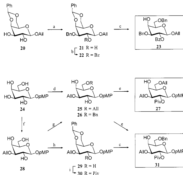
Scheme 2. Synthesis of suitably protected, iterative galactosyl acceptors. Reagents and conditions: a) Bu 2 SnO, toluene, reflux, 16 h, then BnBr, 90 °C, 8 h; 91%. – b) BzCl, DMAP, pyridine/CH 2 Cl 2 , 25 °C, 24 h; 96%. – c) NaBH 3 CN/HCl, Et 2 O/THF, 0 °C, 20 min; 87% ( 23 ); 77% ( 31 ). – d) (Bu 3 Sn) 2 O, toluene, reflux, 16 h, then AllBr/Bu 4 NI, 90 °C, 8 h; 76% ( 25 ). – e) PivCl, Et 3 N, DMAP, pyridine, CH 2 Cl 2 , 25 °C, 12 h; 69% ( 27 ), 78% ( 31 ). – f) Bu 2 SnO, toluene, reflux, 16 h, then AllBr/Bu 4 NBr, THF, reflux, 8 h; 74%. – g) (Bu 3 Sn) 2 O, reflux, 16 h, then AllBr/Bu 4 NI, 80 °C, 8 h; 96% ( 25 ); BnBr/Bu 4 NI, 90 °C, 8 h; 92% ( 26 ). – h) PhCH(OMe) 2 , TsOH, THF, 25 °C, 2 h; 91%. – i) PivCl, DMAP, Et 3 N, CH 2 Cl 2 , reflux, 16 h; 96%. – Abbreviations used throughout: All = allyl, Bn = benzyl, Bz = benzoyl, p MP = p -methoxyphenyl, Ph = phenyl, Piv = pivaloyl
