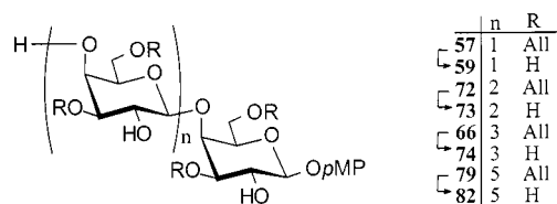
Scheme 7. Removal of allyl ether functionalities by DIBAL in THF/ether or \text{NaBH}_4 in THF/ \text{EtOH} in the presence of \text{NiCl}_2(\text{dppp}) (see ref. [81]) as catalyst
