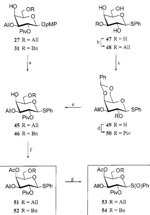
Scheme 4. Generation of \beta -selective galactosyl donors with the selectively removable acetyl blocking group at O -4. Reagents and conditions: a) \text{PhSH} , \text{BF}_3 \cdot \text{OEt}_2 , \text{CH}_2\text{Cl}_2 , 25^\circ\text{C} , 15 min; 79% ( 45 ), 82% ( 46 ). — b) \text{Bu}_2\text{SnO} , toluene, reflux, 16 h, then \text{AlIBr}/\text{Bu}_4\text{NBr} , THF, reflux, 8 h; 68%. — c) \text{PhCH}(\text{OMe})_2 , \text{TsOH} , THF, 25^\circ\text{C} , 2 h; 94%. — d) \text{PivCl} , DMAP, \text{Et}_3\text{N} , \text{CH}_2\text{Cl}_2 , reflux, 16 h; 93%. — e) \text{NaBH}_3\text{CN}/\text{HCl} , \text{Et}_3\text{O}/\text{THF} , 0^\circ\text{C} , 20 min; 82%. — f) \text{Ac}_2\text{O} , \text{Et}_3\text{N} , DMAP, \text{CH}_2\text{Cl}_2 , 25^\circ\text{C} , 2 h; 94% ( 51 ), 93% ( 52 ). — g) m CPBA, \text{CH}_2\text{Cl}_2 , -78^\circ\text{C} , 15 min; 84% ( 53 ), 92% ( 54 ). — p MP = p -methoxyphenyl
