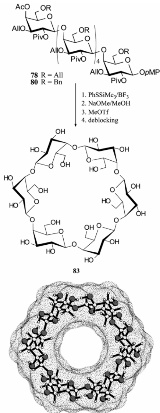
Scheme 8. Conceptual approach to a hexameric \beta(1\rightarrow4) -cyclogalactin 83 , an “inside-out” analogue of \alpha -cyclodextrin, possessing a slightly wider, less hydrophobic cavity, based on calculations of its solvent-accessible surface (given in dotted form with a ball-and-stick model insert) and molecular lipophilicity distribution (see refs. [29, 30])
