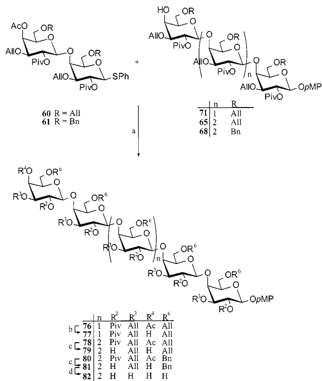
Scheme 6. Synthesis of \beta(1\rightarrow4) -galactopenta- and -hexasaccharides. Reagents and conditions: a) MeOTf, DTBMP, 4 Å molecular sieves, \text{CH}_2\text{Cl}_2 , 25 °C, 16 h; 67% ( 76 ), 77% ( 78 ), 78% ( 80 ). – b) \text{NaOMe}/\text{MeOH} , 25 °C, 16 h; 88%. – c) \text{LiOH}/\text{MeOH} , reflux, 16 h; 89% ( 79 ), 86% ( 81 ). – d) DIBAL/ [\text{NiCl}_2(\text{dppp})] , THF/ \text{Et}_2\text{O} , 0 \rightarrow 25 °C, 16 h \rightarrow \text{Ac}_2\text{O}/\text{DMAP}/\text{pyridine} , 40 °C, 4 h \rightarrow \text{H}_2 , Pd/C, AcOH, 25 °C, 5 h \rightarrow \text{NaOMe}/\text{MeOH} , 25 °C, 6 h; 64%
