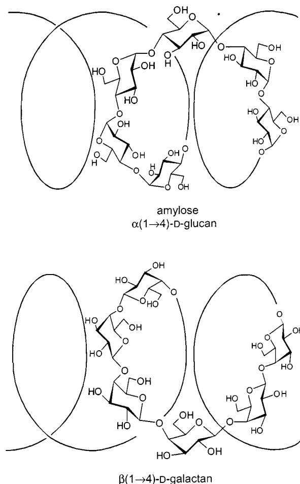
Figure 1. Sketched representation of a left-handed, single stranded helix of V_H -amylose (top) and a right-handed \beta(1\rightarrow4) -D-galactan helix (bottom), both free of steric constraints as predicted by early computational studies (see refs. [20–24] )
